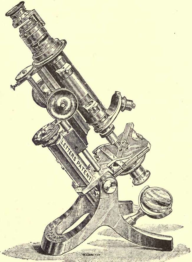
Fig. 15.—Petrological microscope with fixed stage and rotating nicols and cross-wires
